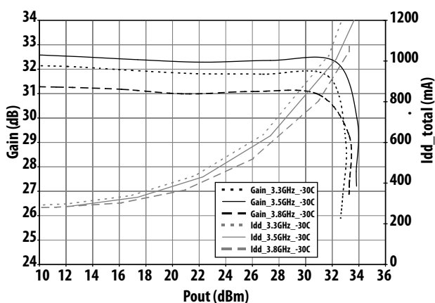
Figure 11. CW Gain vs Pout @ -30°C, high-gain mode, Vdd = 5V
