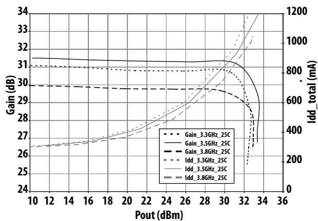
Figure 9. CW Gain vs Pout @ 25°C, high-gain mode, Vdd = 5V
