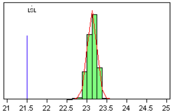
Figure 1a. Linear Pout Distribution (normal gain mode)
